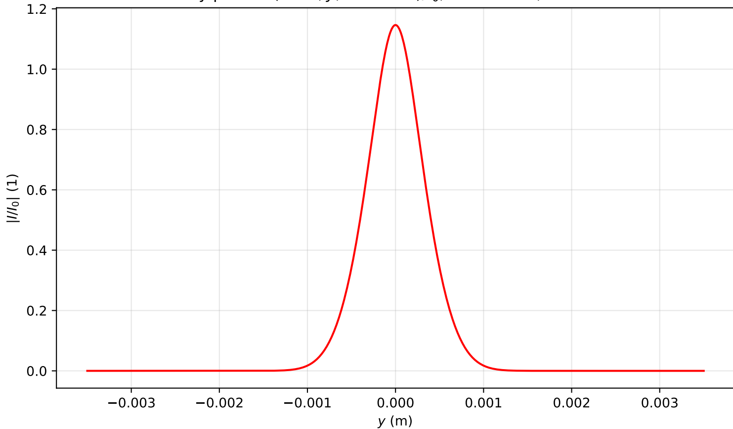
Intensity profile I(x=0, y, z=0.239)/I_0 , \text{Pin}=2.5\text{Pcr} , artificial time
